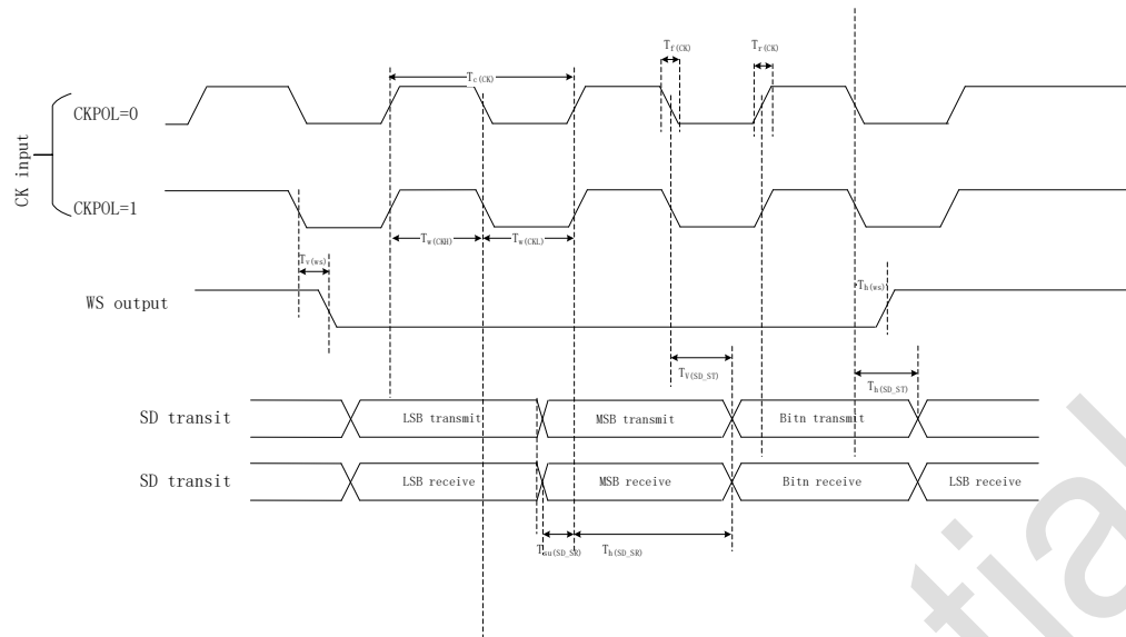
Figure 5-9 I 2 S master timing diagram (Philips protocol)
