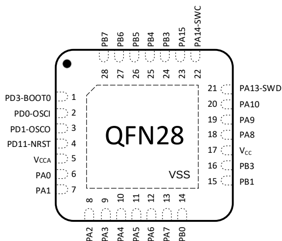
Figure 3-5 QFN28 (4*4) PY32F410G1xU7 Pinout1 (Top view)
